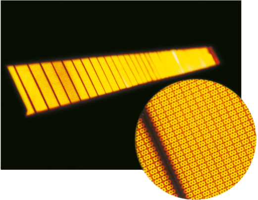
Maintenance free ceramic gas burner minimizes downtimes. 20% more efficient than regular blue flame burners. A unique and patented burner by Electrolux Professional.
